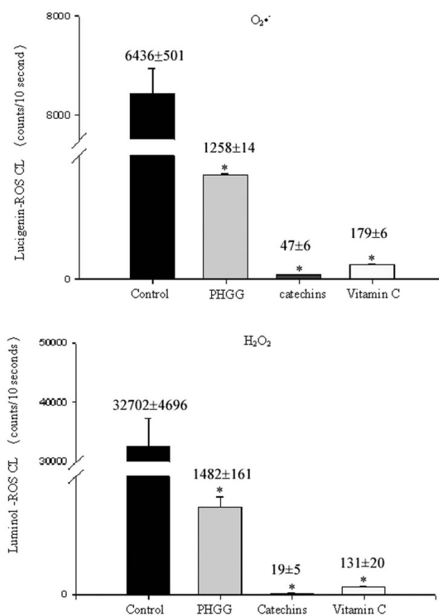
Figure 2 The antioxidant activity against O_2^{\cdot-} , H_2O_2 , HOCl in control (distilled water), PHGG, catechins and vitamin C is demonstrated. Catechins, vitamin C and PHGG significantly reduced O_2^{\cdot-} , H_2O_2 , HOCl activity in an order of catechins > vitamin C > PHGG > control. Each test was performed 6 times. * P < 0.05 when compared to the control value.
