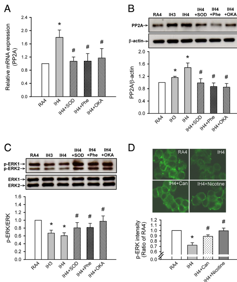
Figure 2 Intermittent hypoxia (IH) effects on protein phosphatase 2A (PP2A) and extracellular signal-regulated kinase 1/2 (ERK1/2) phosphorylation. (A) PP2A mRNA levels were determined by real-time quantitative polymerase chain reaction (qPCR) and (B) PP2A protein levels were determined by Western blot in PC12 cells after 4 days of room air exposure (RA4, n = 7), 3–4 days of IH (IH3, n = 5; IH4, n = 5), and IH4 along with superoxide dismutase (IH4 + SOD, n = 6), 1,10-phenanthroline (IH4 + Phe, n = 5) or okadaic acid (IH4 + OKA, n = 5). (C) ERK1/2 phosphorylation levels in PC12 cells were determined by Western blotting after RA4, IH3, IH4, IH4 + SOD, IH4 + Phe, IH4 + OKA and (D) immunocytofluorescence (green) after RA4, IH4, IH4 along with cantharidin (IH4 + Can, n = 5) and nicotine (IH4 + Nicotine, n = 5). * p < 0.05 compared with RA4. # p < 0.05 compared with IH4. Values are means \pm SEMs.
